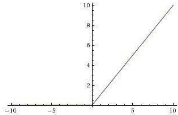
Fig.5. Relu non-linearity
